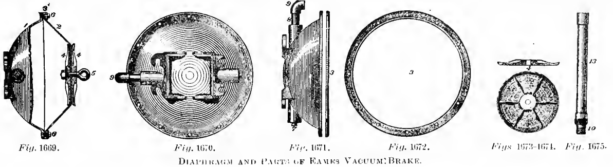
DIAPHRAGM AND PARTS OF EAMES VACUUM BRAKE.
